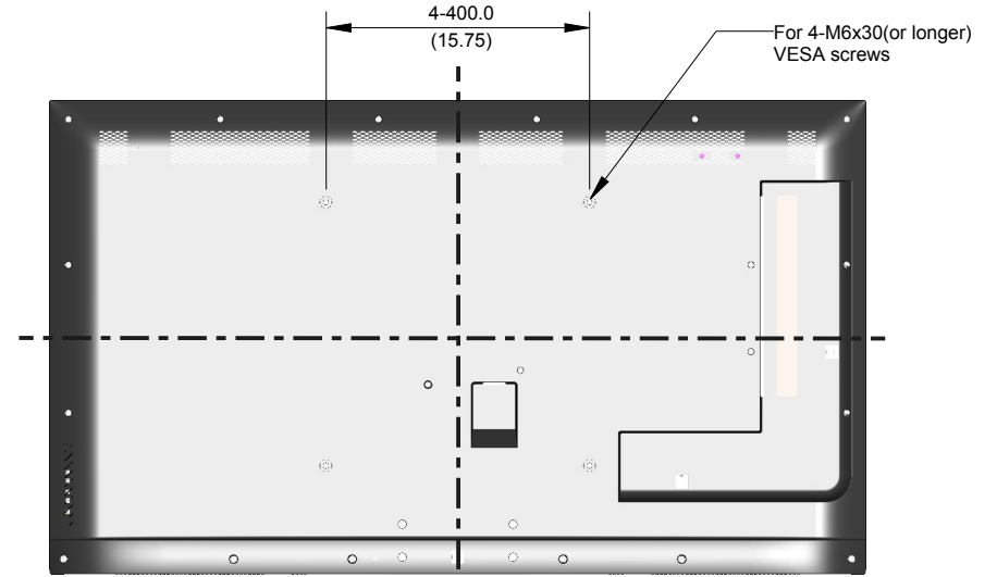
Back View of Monitor without Stand
